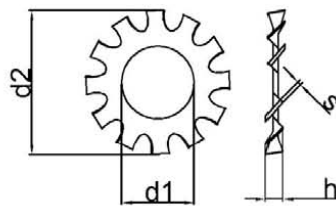
Type A externally toothed
