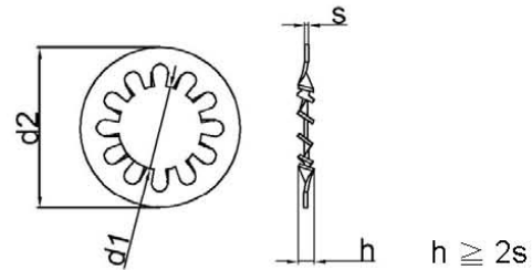
Type J internally toothed
